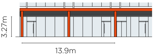
Central Square Elevation - Unit 4
