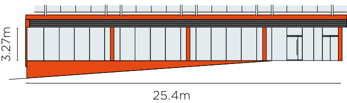
Ecclestone Bridge Elevation - Unit 1
