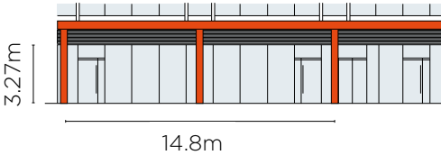
Buckingham Palace Elevation - Unit 2-3
